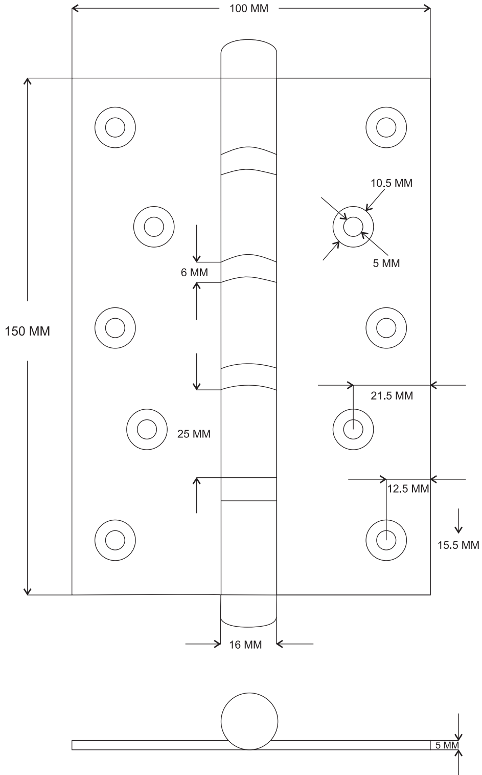
Brass Ball Rearing Hinges Size : 150 x 100 x 5MM Madhuram Overseas
